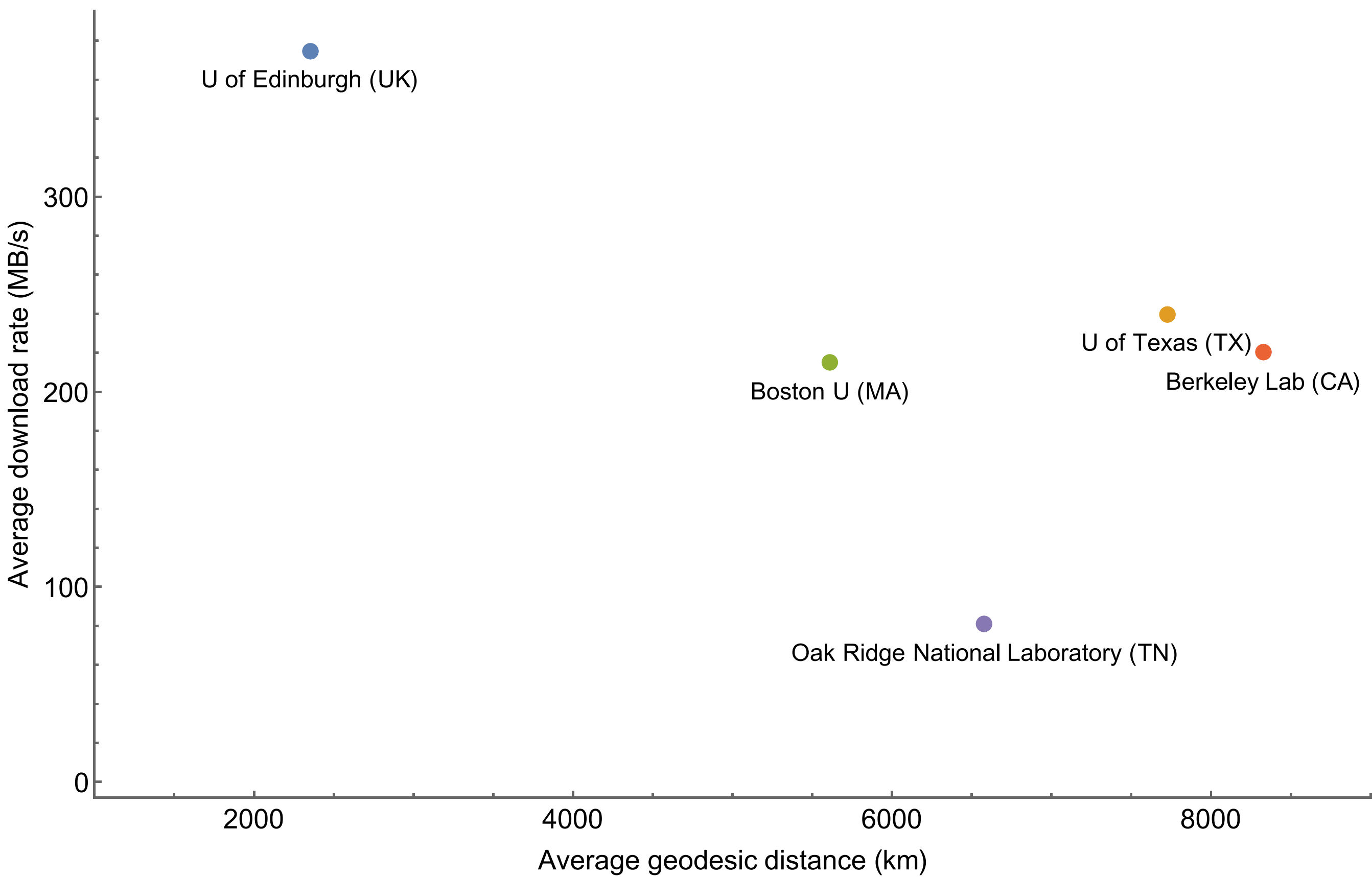
Figure 8 - Average download rate in MB/s vs. average geodesic distance between the download location and file pieces locations on Storj DCS.
